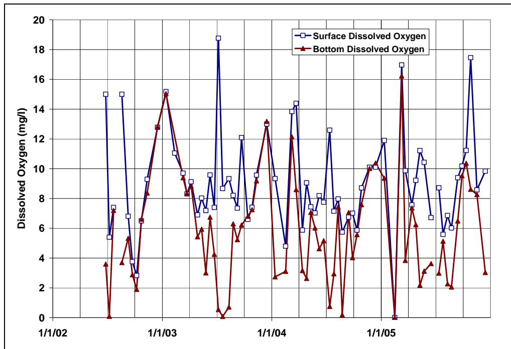
Figure 10. Surface and Bottom Dissolved Oxygen Concentrations in Milton Reservoir (Station M3)
